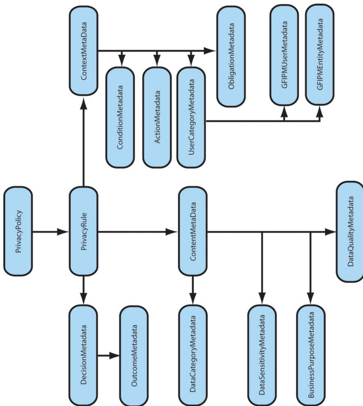
Figure 4: Privacy Policy Metadata Model
